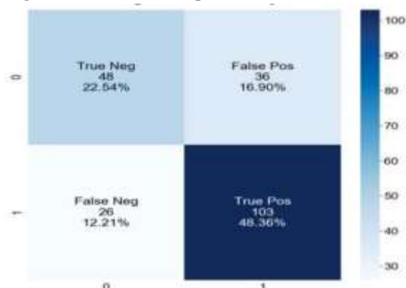
Fig. 5. Confusion Matrix
