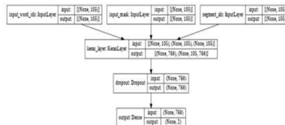
Fig.1. BERT model based on sentiment analysis The Fig.1 depicts the BERT model we developed for sentimental analysis. The three separate embeddings are summarized together to give input to the internal layers of the model. The Fig.2 demonstrates the flow of the sentimental analysis process. To begin with, the final CLS token will output a matrix of hidden size. Furthermore it will be passed to a classifier layer. In conclusion the classifier layer will determine the sentiment of the input text.
