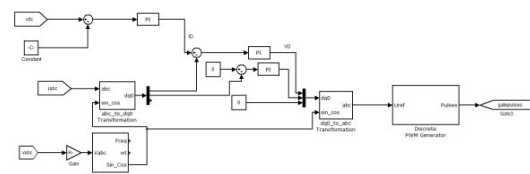
Fig.3.3 proposed controller.
