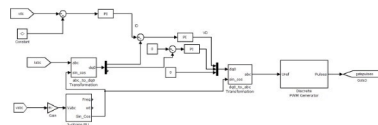
Fig.3.6 proposed controller.
