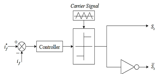
Fig.3.7 The Principle of Sinusoidal PWM Control Method
