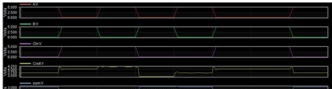
Fig:8 Timing waveform of full adder design with XOR and NAND gate using 45 nm technology.
