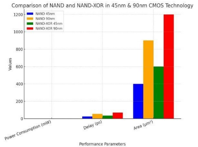
Graph:2 Performance Comparison of Different CMOS Technologies
