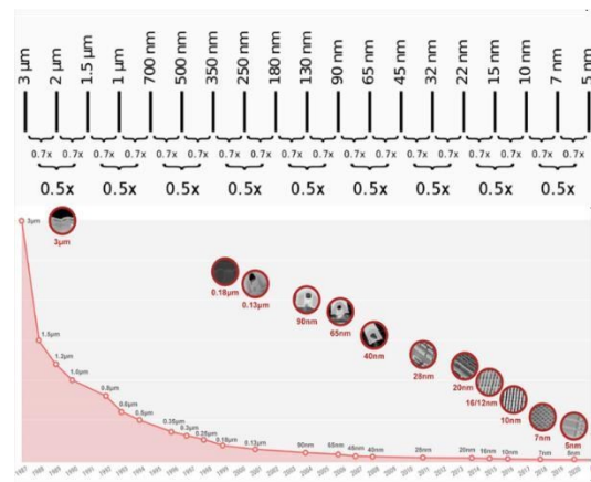
Fig:3 Technology nodes
