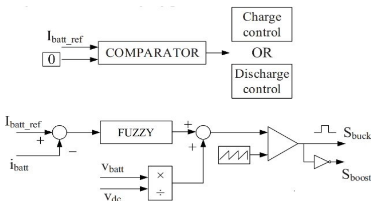
Fig. 6. Current Battery Charger Control Strategy Inverter Control
