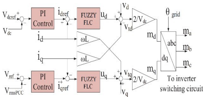
Fig. 8. Inverter control system.
