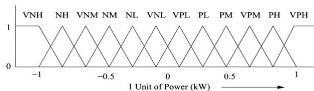
Fig. 11. Fuzzy membership function-load/source of EV battery.
