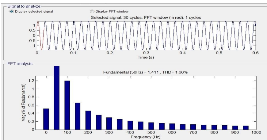
Fig. 17. PI controller harmonic spectrum and THD of grid injected current.
