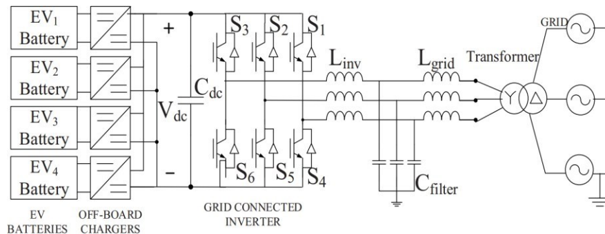
Fig. 4. EV charge station for quick dc load.
