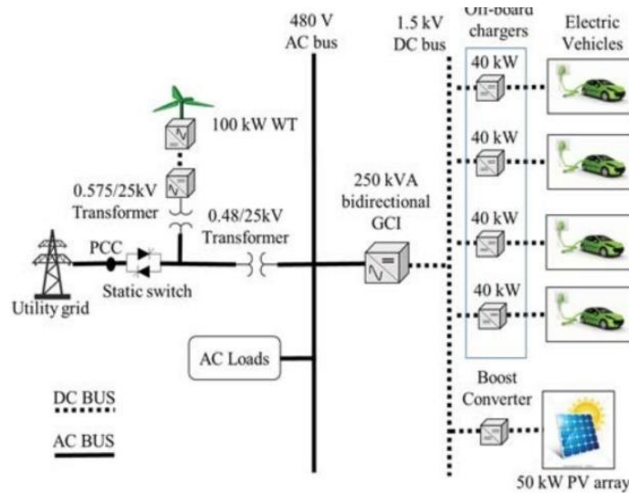
Fig. 13. Proposed microgrid test system configuration.
