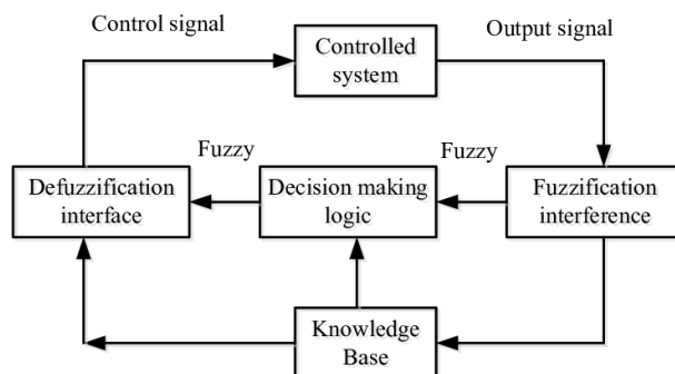
Fig. 7: FLC system.
