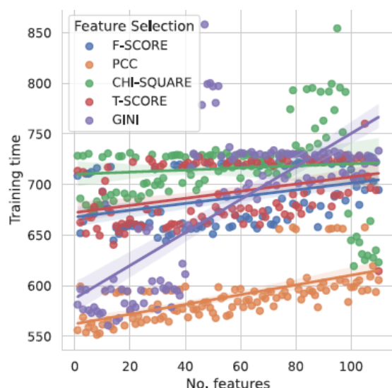
Fig. 1: Training time as a linear approximation function of the number of features ranked according to the feature selection strategy adopted.
