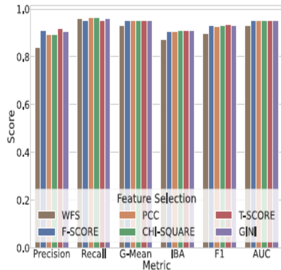
Fig. 4: Classification metric scores derived from Fig. 3.
