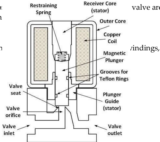
Figure 1 Cross section view of the proportional solenoid valve
