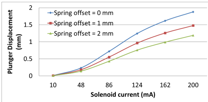
Figure 31 Effective plunger displacement vs solenoid current characteristics of the flat non-optimal design with various offsets
