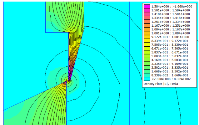
Figure 22 Magnetic flux density plot of the optimized proportional solenoid geometry in FEM
