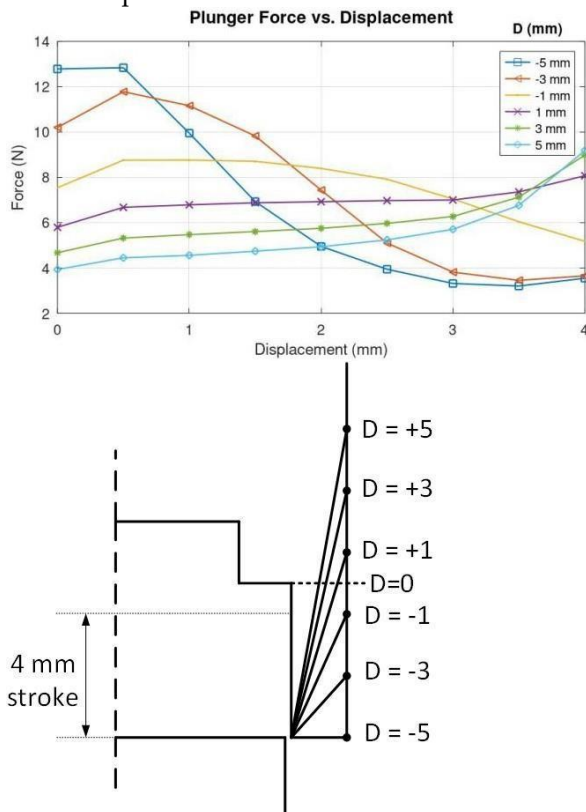
Figure 4 Optimization of D in the first iteration
