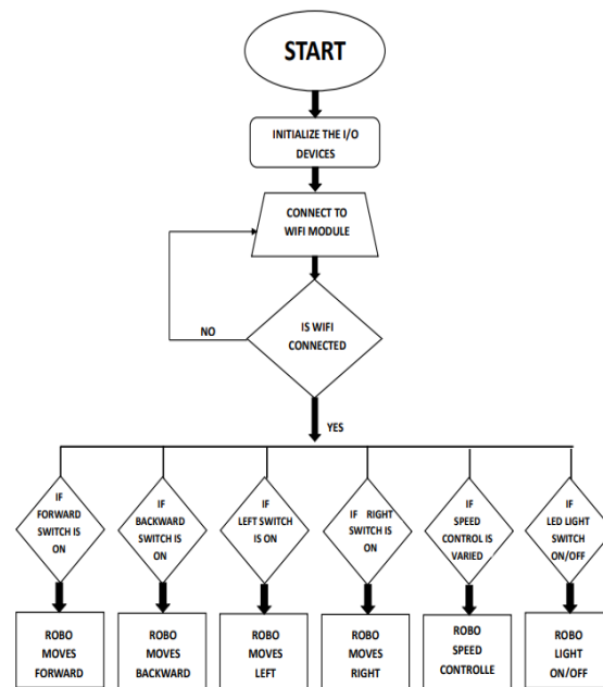
Figure.3 Flow Chart
