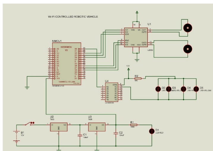
Figure.2 Schematic Diagram
