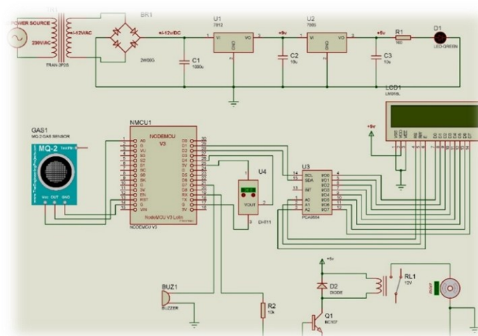
Figure.3 Schematic diagram
