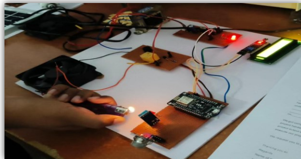
Figure.6 Fire Detection
