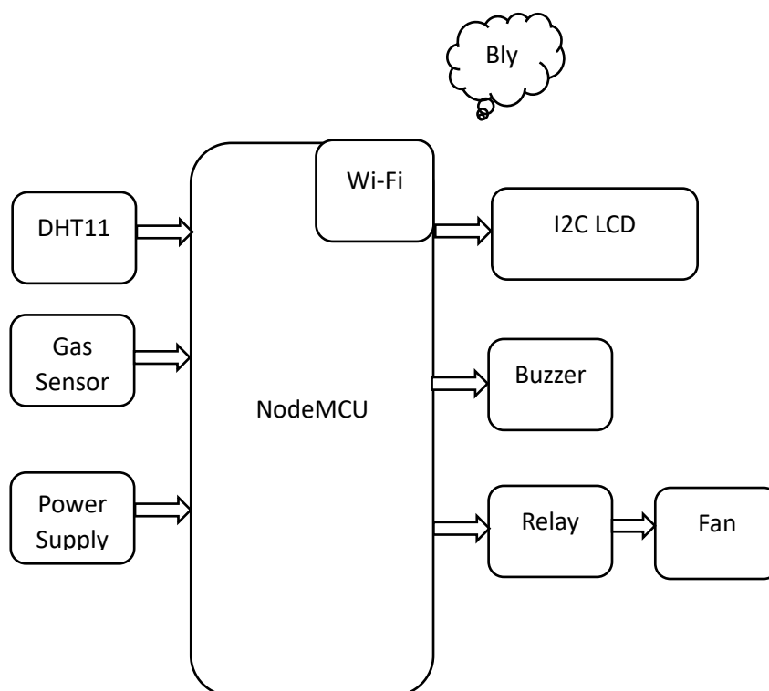
Figure.1 Block Diagram
