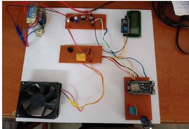
Figure.4 Hardware Working kit
