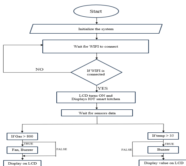
Figure.2 Flow Chart
