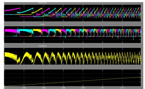
Fig 6.6 Scope 2 Result
