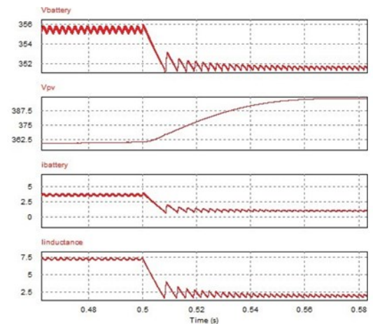
Fig.6.4.PVchargingmode6
