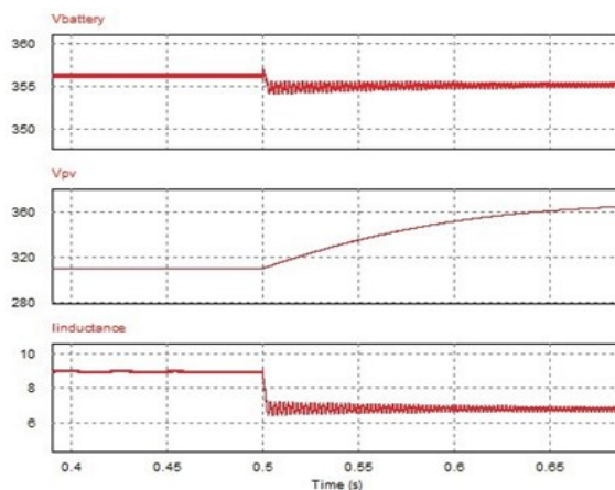
Fig. 6.3.Simulation results for charging modes Gridcharging.
