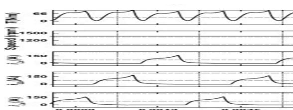
Fig.6.2.Simulationresultsofsingle-sourcedrivingmode
