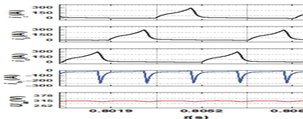
Fig.6.1.Simulationresultsofdriving-chargingmode
