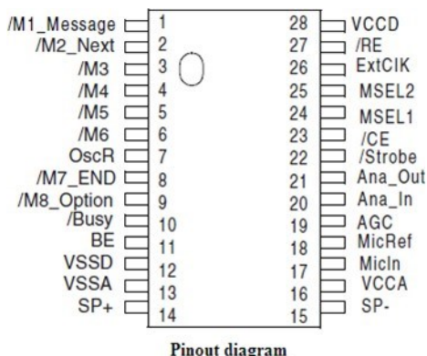
Fig.3 Functional unit of APR9600
