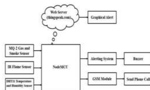
Fig. 3.1 - Overall working diagram of the proposed system.
