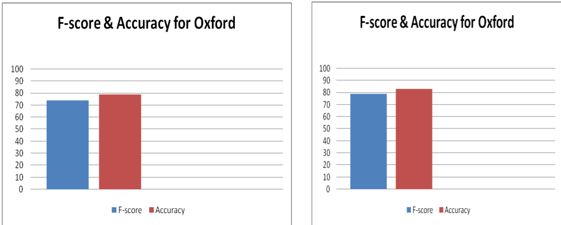
a) F-score and accuracy before the application of fuzzy b) F-score and accuracy after the application of fuzzy
