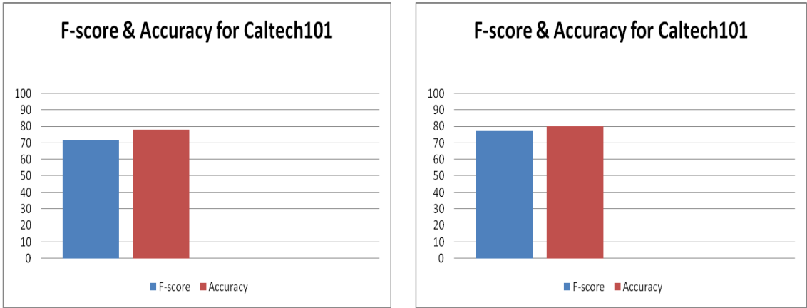
a) F-score and accuracy before the application of fuzzy b) F-score and accuracy after the application of fuzzy
