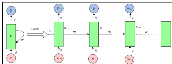
Fig.1. RNN Architecture
