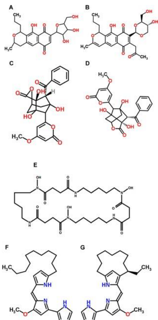
Figure 1. Compound structures.
