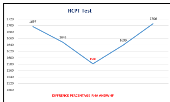
Figure 4: RCPT 56 days coulombs
