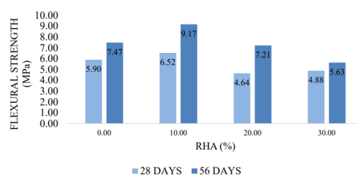
Figure 3: Flexural strength test results of 28 and 56 days of curing
