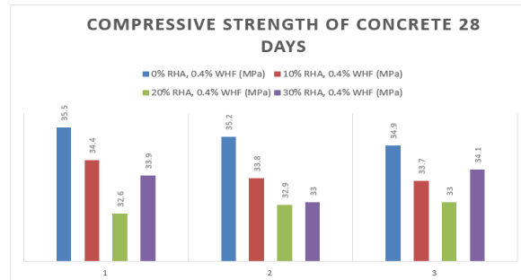
Figure 1: compressive strength of concrete
