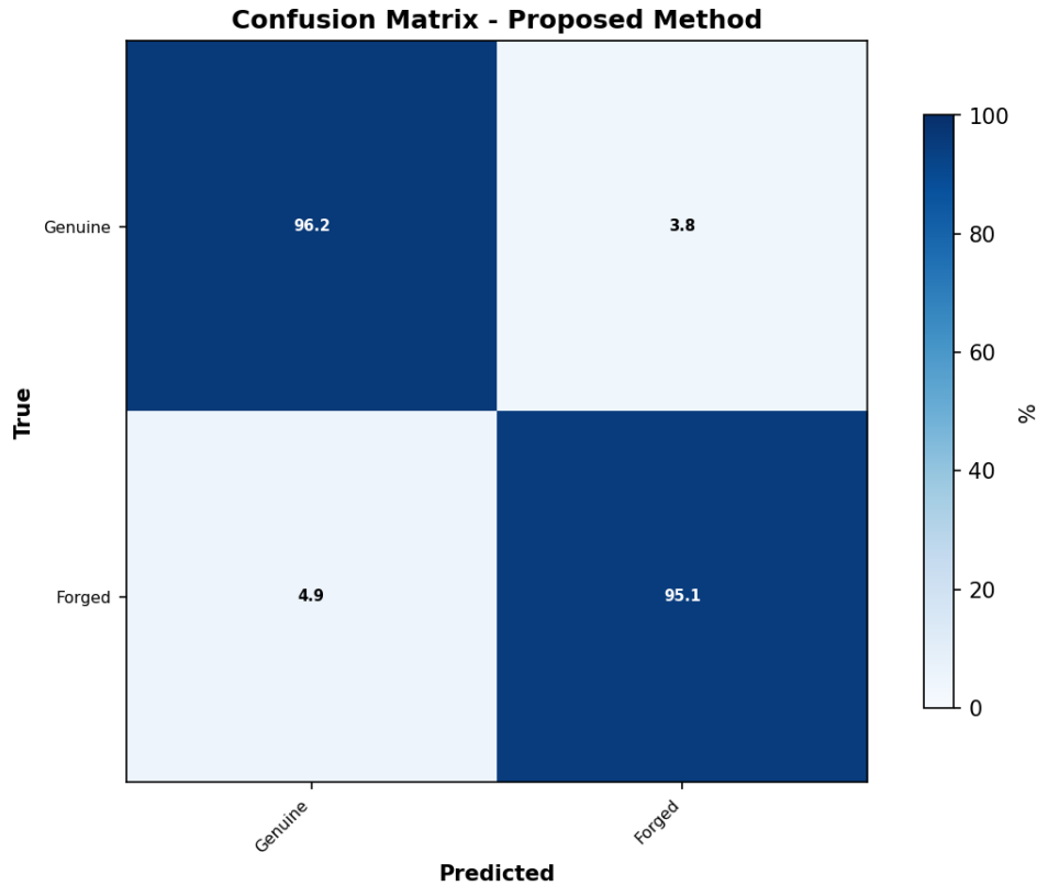
Figure 5: Confusion Matrix for SigVerify on the Test Set. Diagonal values represent correct classification rates.
