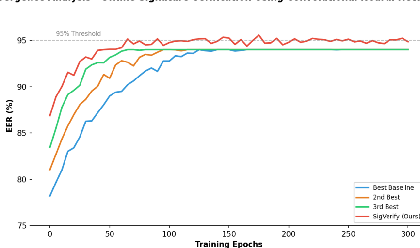
Figure 4: Convergence Analysis. SigVerify reaches 95% at epoch 135, faster than baselines.
