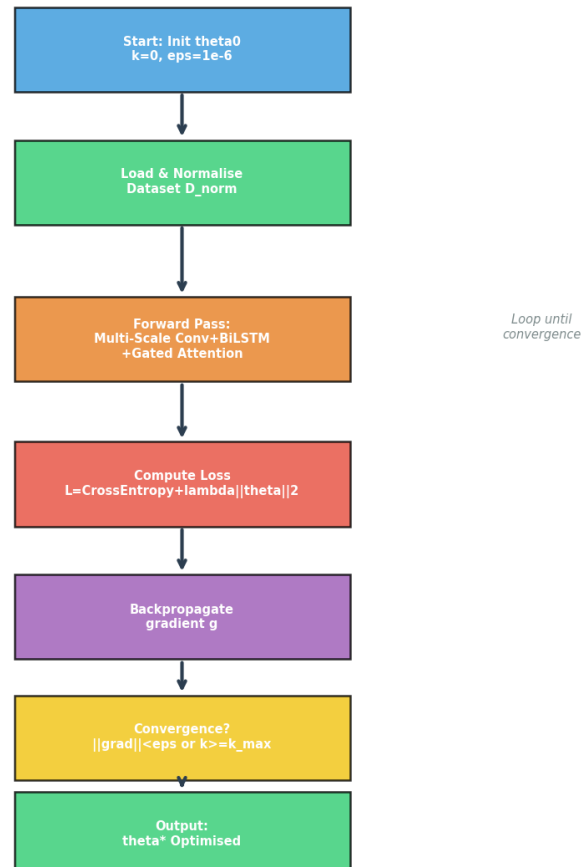
Figure 2: Algorithmic Flowchart of the SigVerify Training Procedure. Step numbers correspond to Algorithm 1.
