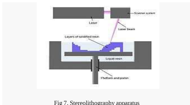
Fig 7. Stereolithography apparatus
