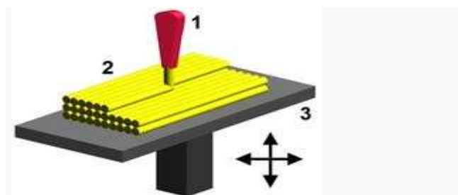
Fig 4. Extrusion deposition
