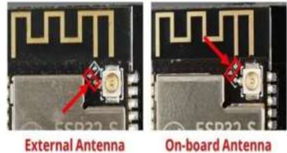
Figure 6: Antenna
