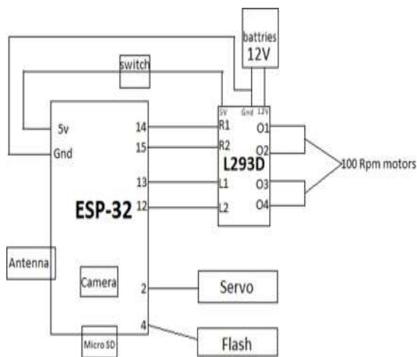
Figure 1: Block Diagram
