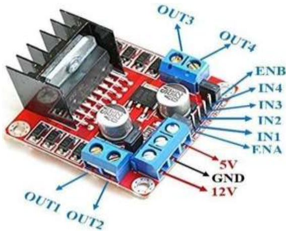
Figure 3: Motor Driver
