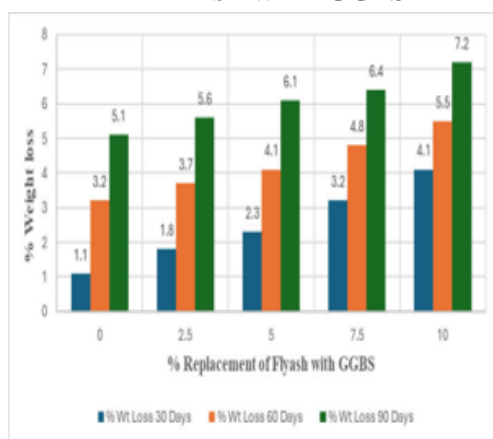
GRAPH-4- WEIGHT LOSS OF GEOPOLYMER CONCRETE MADE BY REPLACEMENT OF FLYASH WITH GGBS
