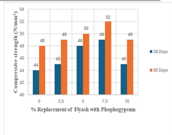
GRAPH-2- COMPRESSIVE STRENGTH OF GEOPOLYMER CONCRETE MADE BY REPLACEMENT OF FLYASH WITH PHOSPHOGYPSUM
