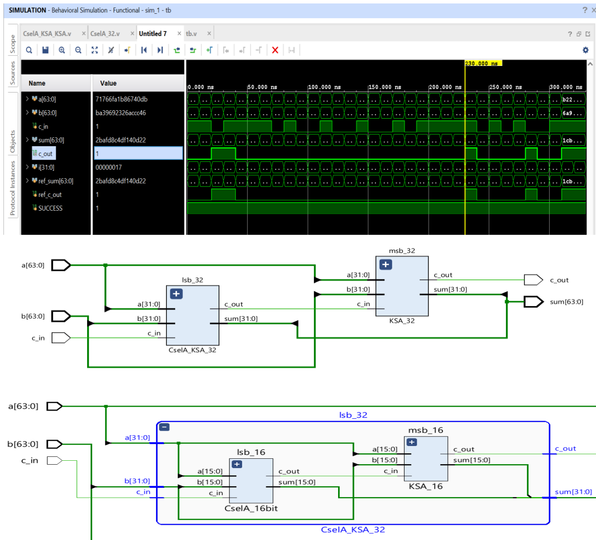
Fig 9 Simulation waveform of Hybrid Adder ((CSeLA(16-bit) + KSA (16-bit)) + KSA (32-bit))
