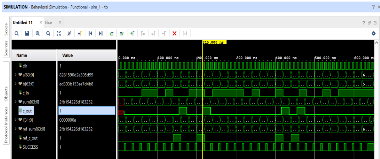
Fig 2 Simulation waveform of Ripple Carry Adder (64-bit)
