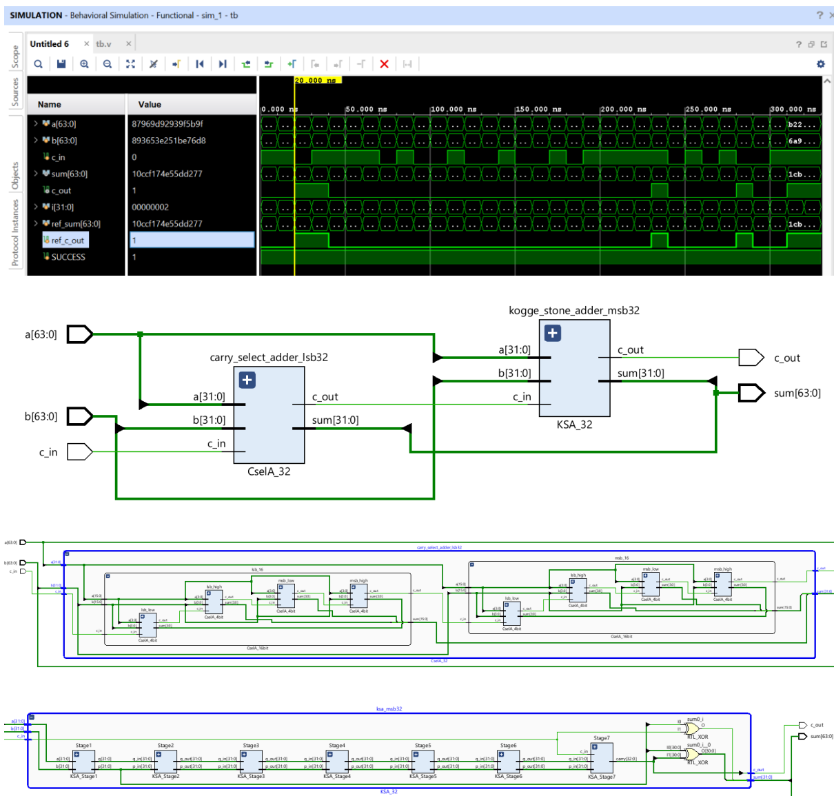
Fig 8 Simulation waveform of Hybrid Adder (CSeLA(32-bit) + KSA (32-bit))
