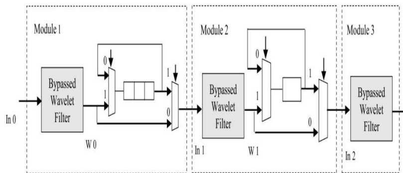
Fig 3: Overall DWPT Architecture
