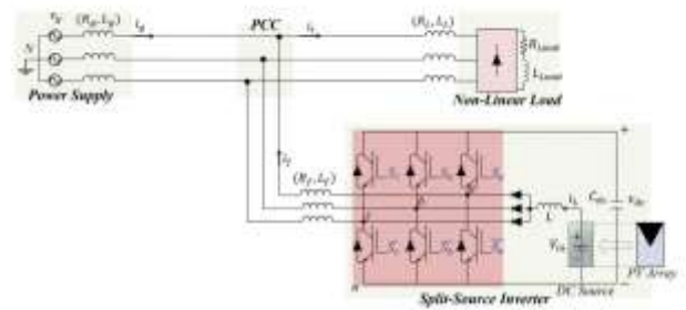
FIGURE 1. Multifunctional grid-connected system based-split-source inverter.
