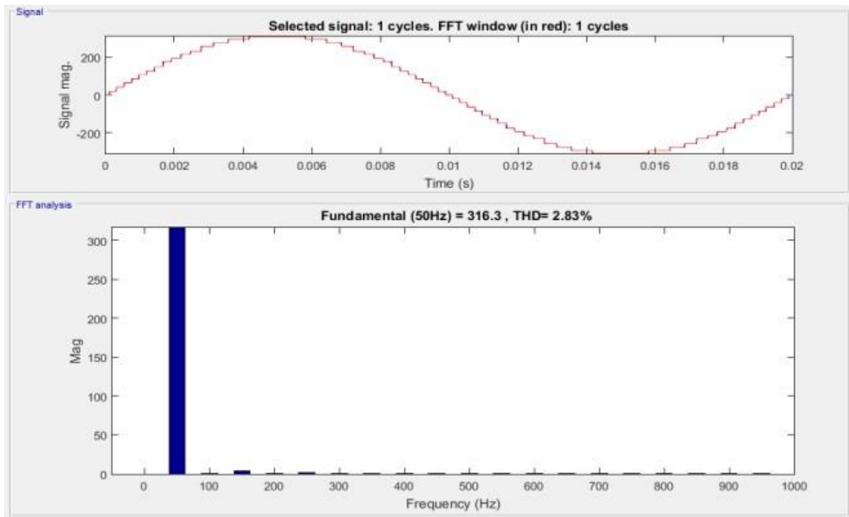
Fig. 6. Harmonic waveform and output voltage waveform simulated
