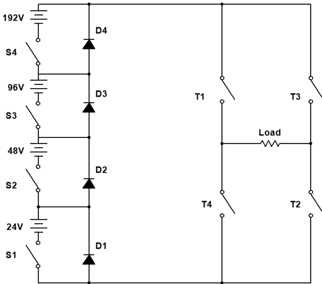
Fig. 3. Circuit Diagram
