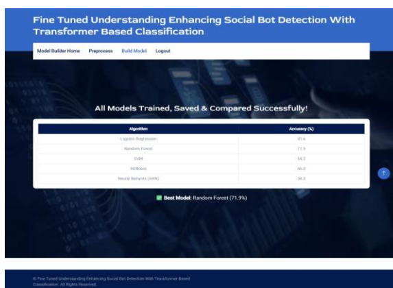
Fig 6.3: Algorithms
