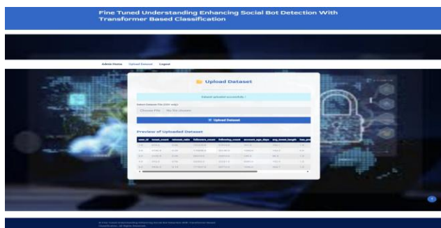
Fig 6.2: Dataset
