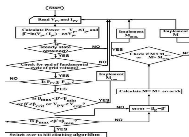
Fig 3.2: MPPT algorithm for \beta -method
