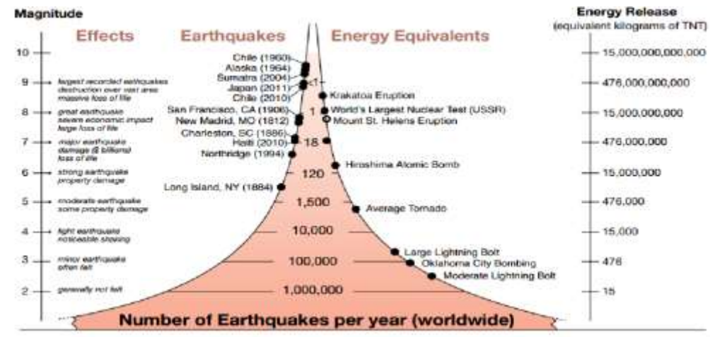
Fig 1: Number of Earthquake per year
