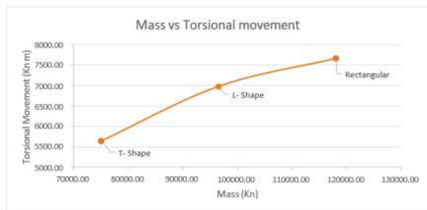
Fig 6: Mass v/s Torsional Movement
