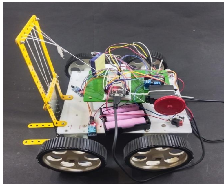
Figure.2 Practical device
