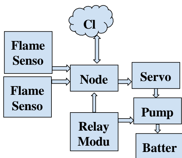
Figure 3.1: Block Diagram
