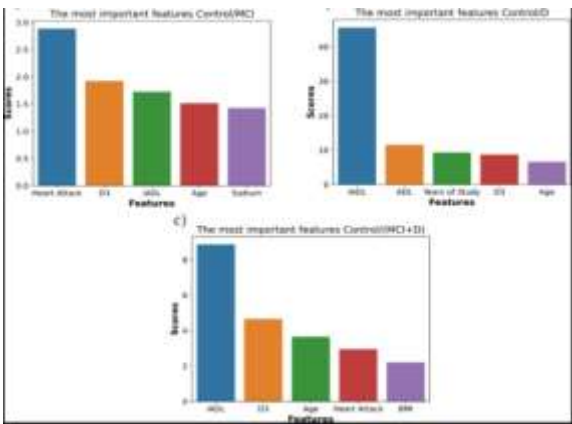
Figure 3: Feature Importance Analysis of Cognitive Parameters
