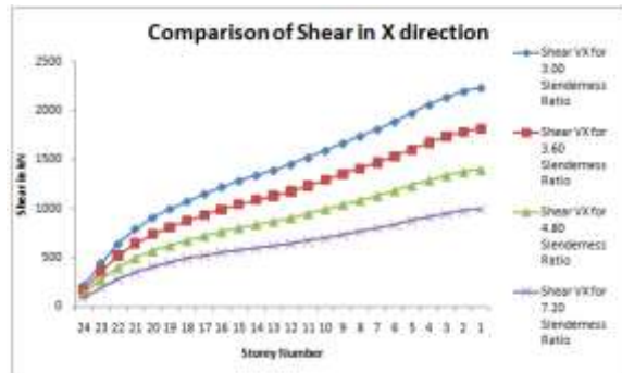
Comparison of Shear Vx
