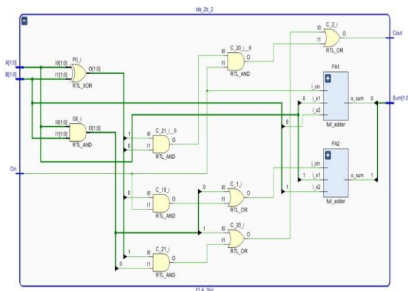
Figure.3 CLA
