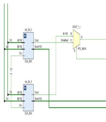
Figure.4 CLA MUX
