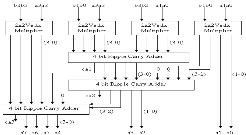
Figure.1 Block Diagram of 4x4 bit Vedic Multiplier
