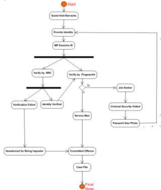
Figure.3: Activity Diagram
