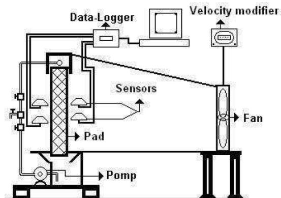
Figure 2. Experimental set.
