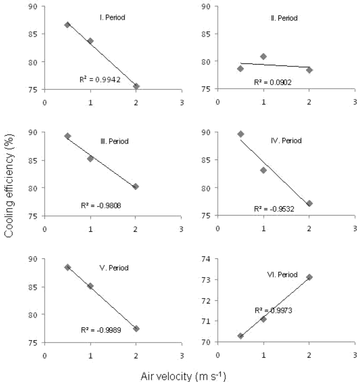
Figure 3. Correlation values about the relationship between velocity of air passing through the pad and calculated cooling efficiency in different periods.
