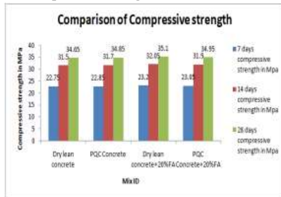
Graph 2: Comparison of compressive strength
