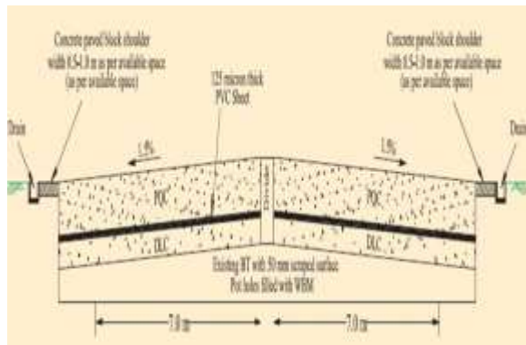
Fig 1: Typical cross-section of the concrete road
