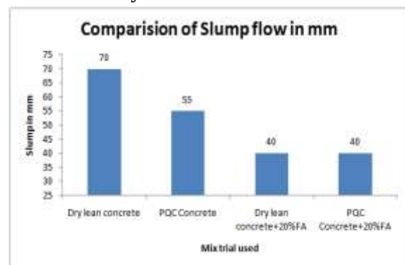
Graph 1: Comparison of slump cone test results
