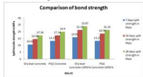
Graph 5: Comparison of bond strength of concrete
