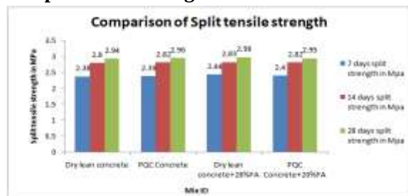
Graph 3: Comparison of split tensile strength
