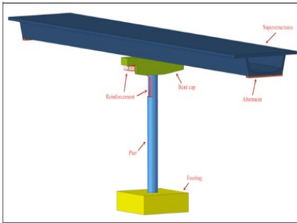
Figure 11. Specific sizes of the pier models.
