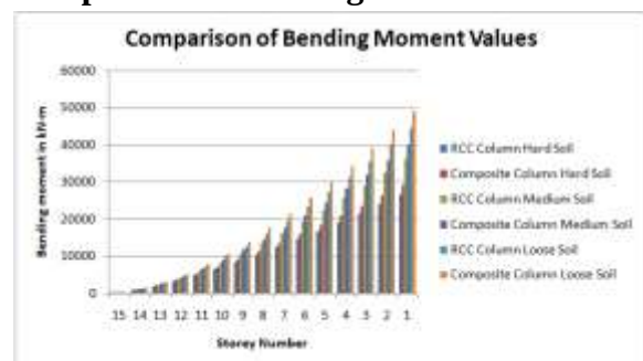
Comparison of bending moment
