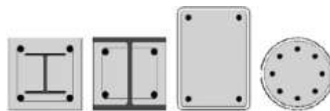
Typical composite column cross sections
