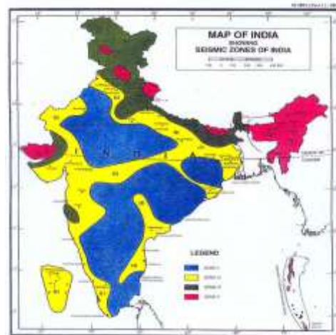
Seismic zone map in India
