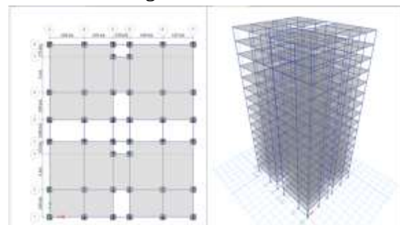
Composite column Building
