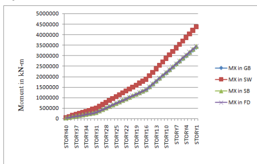
Storey Moment in X-Direction for Zone III Storey Moment in Y-Direction for Zone III
