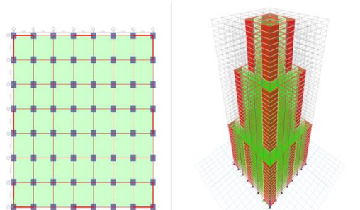
Model retrofitted with shear walls
