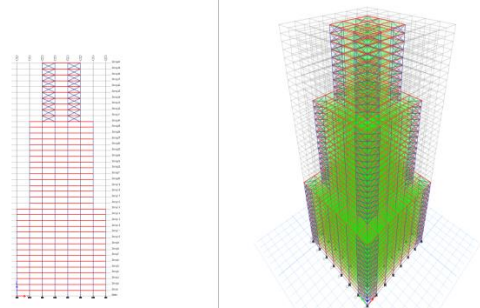
Model retrofitted with steel bracings
