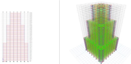
Model retrofitted with friction dampers
