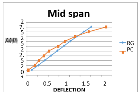
Load Deflection Curves At 7 Days @Mid Span
