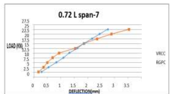
Load Deflection Curves @ 7 Days @ 0.72 L
