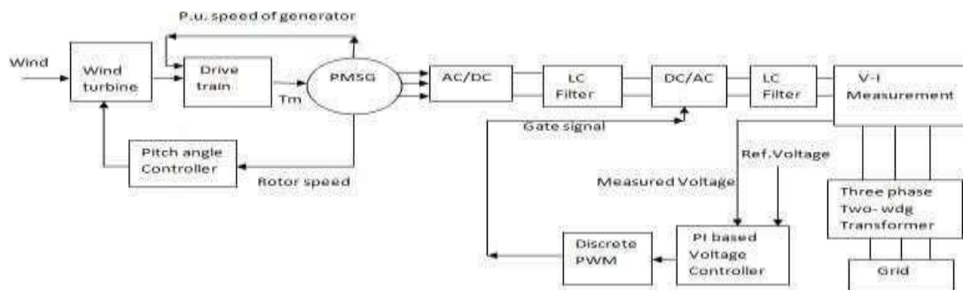
Fig. 4. Block diagram of grid connected PMSG based wind turbine system
