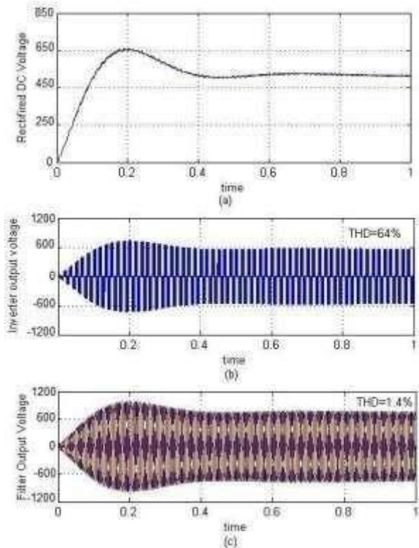
Fig. 9. (a) Rectified dc voltage (b) inverter output voltage and (c) filter output voltage
