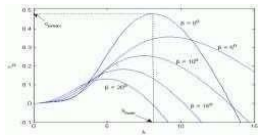
Fig. 1. C_p - \lambda curve.
