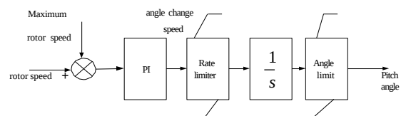
Fig. 3. Pitch Angle Controller Model
