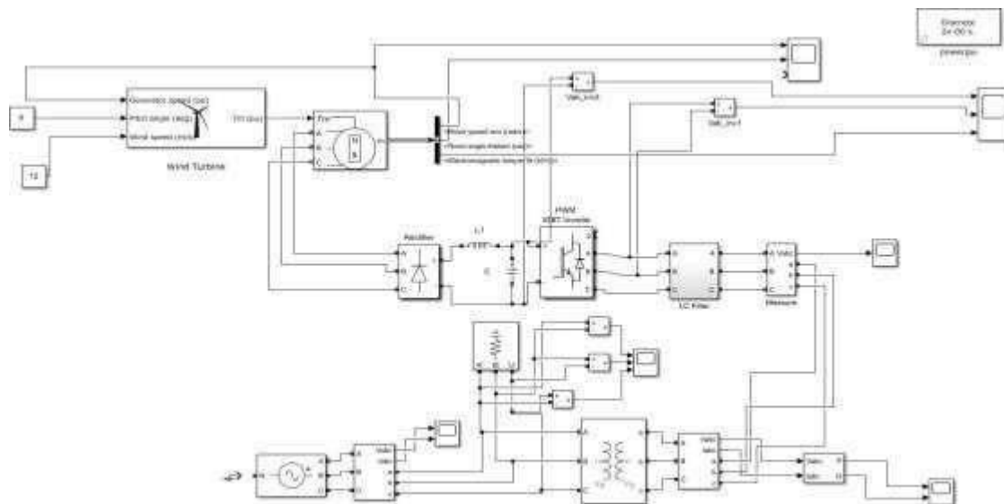
Fig. 4. Block diagram of grid connected PMSG based wind turbine system
