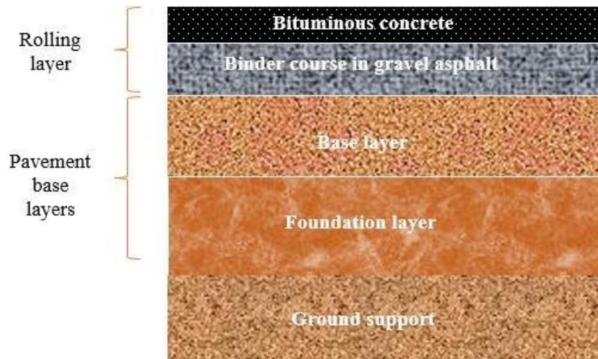
Figure 2: Typical section of flexible pavement
