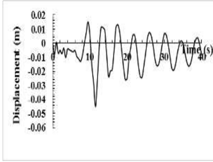
Figure 12. Displacement-time history of dam crest
